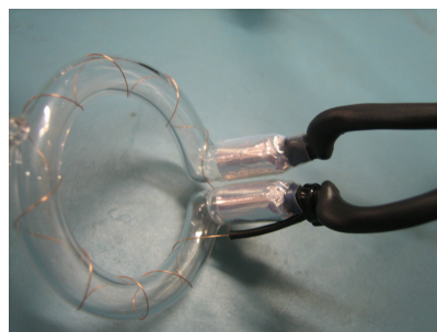
Figure 7: Trigger electrode for flash lamp
