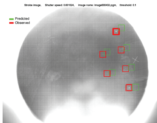
Figure 28: Rectangular markers showing the positions of the reflective crosses and the retro-reflectors superimposed onto the raw strobe-image
