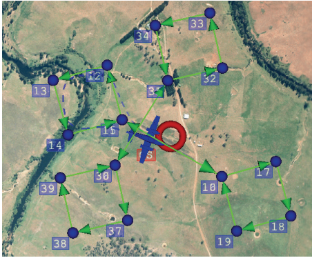
Figure 20: Aerial image of the test site at Marulan with the flight paths overlaid. The two dumbbell circuits are defined by waypoints 10 to 19 and 30 to 39.
