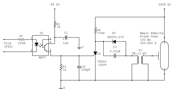
Figure 6: Strobe trigger circuit
