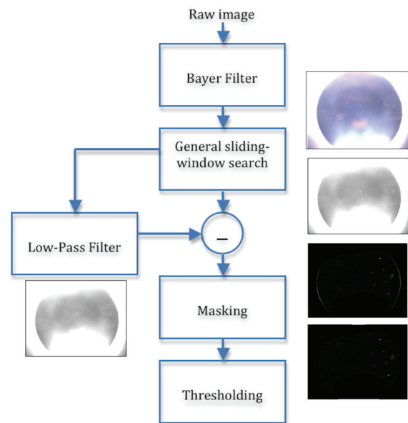
Figure 27: Processing applied to a strobe-image
