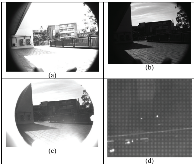
Figure 14: Images for a camera aperture of f4. a) Shutter speed optimised for ambient light b) Shutter speed set to 0.5ms c) Strobe image with shutter speed set to 0.5ms d) Expanded view showing retro reflector returns at 125m
