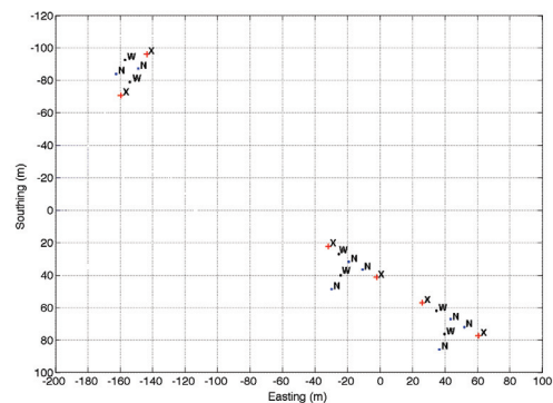
Figure 19: Navigation solution showing the surveyed positions of the crosses and the retro-reflectors
