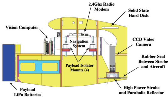
Figure 17: Installation of the Strobe/Camera system in the UAV
