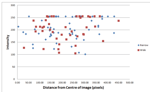
Figure 25: Measured intensity of the light reflected from the retro-reflectors as a function of their angle
