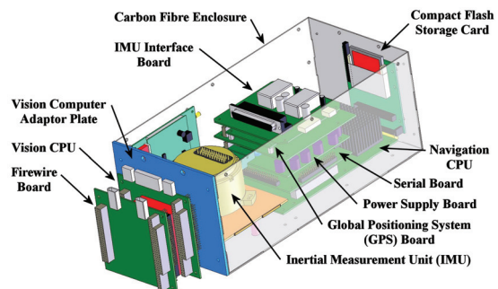
Figure 16: Graphic showing the navigation and vision payload module installed in the UAV
