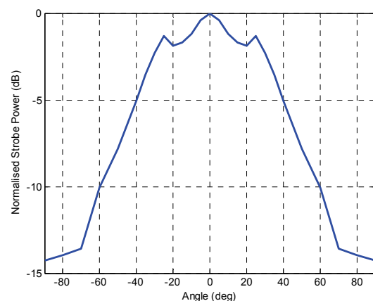
Figure 12: Measured angular field of view of the strobe
